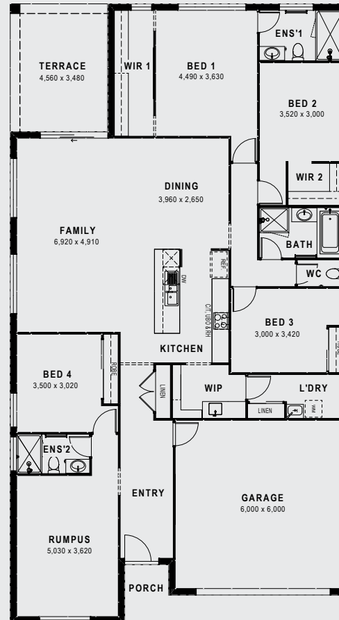
DESIGNER - 260.93m 2 / 28.09sq
