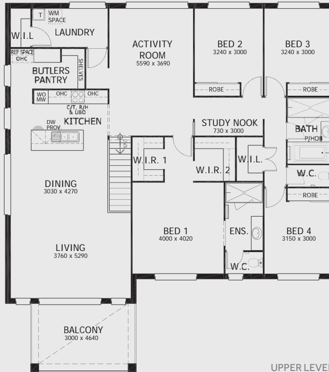
UPPER LEVEL
